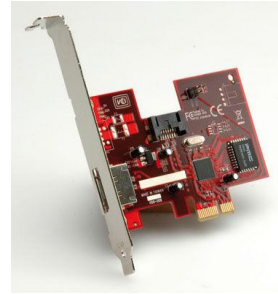
Adaptador PCI-Express 1 + 1 x SATA II - AVD. PCI-Express Adapter, 1 + 1 x SATA II Ports - AVD.
